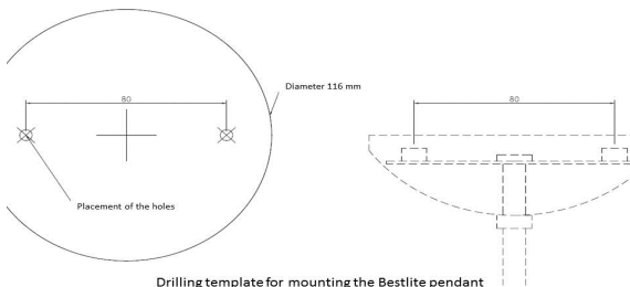
Drilling template for mounting the Bestlite pendant
